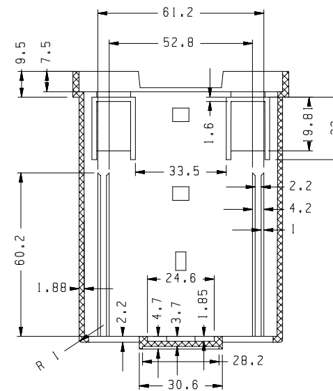
SECTION J - J
